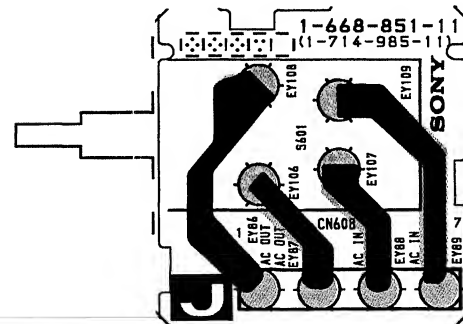
- J BOARD -
