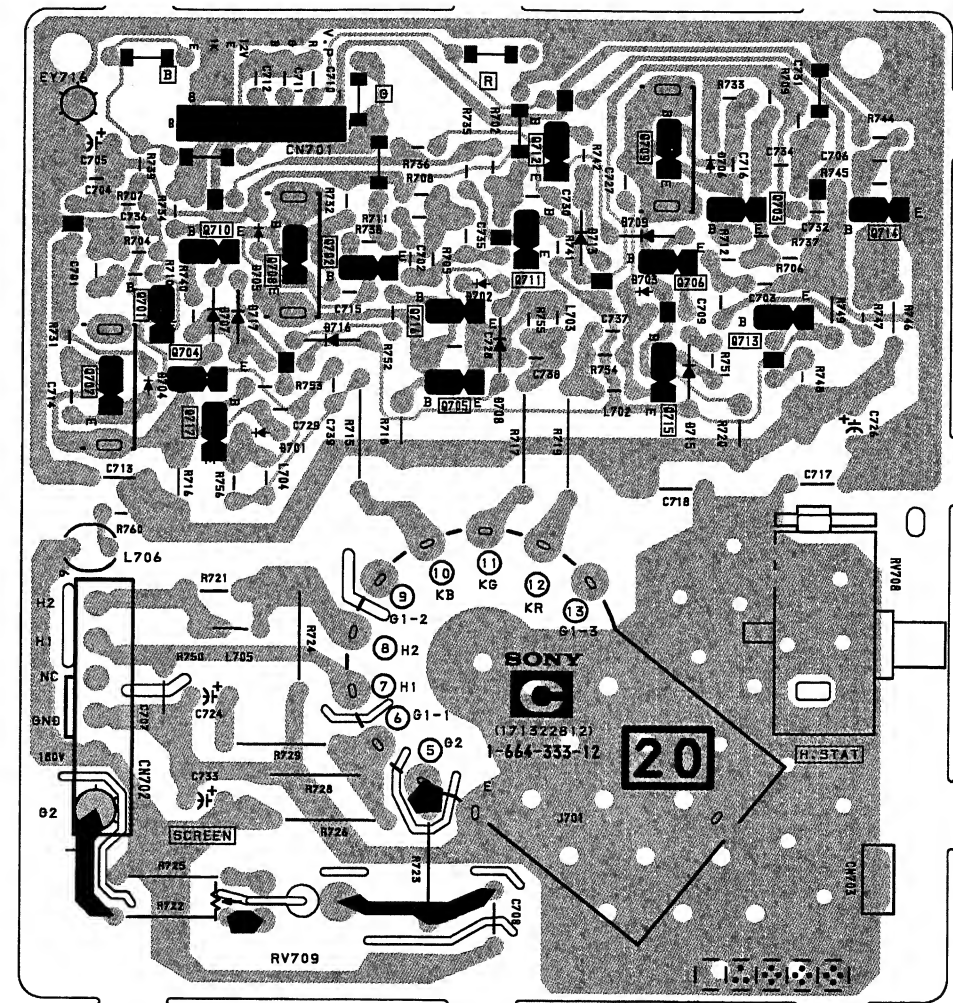
- C BOARD -
