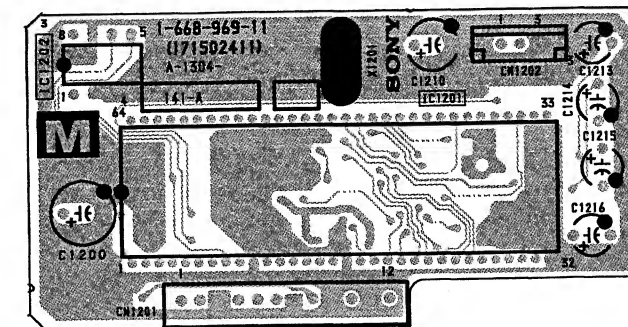
- M BOARD - <A Side>
