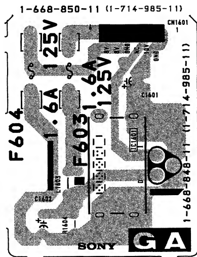
- GA BOARD -
