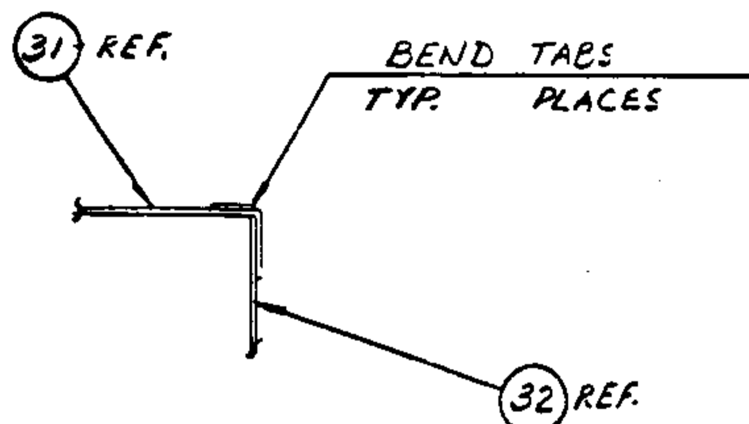
DETAIL "X"
