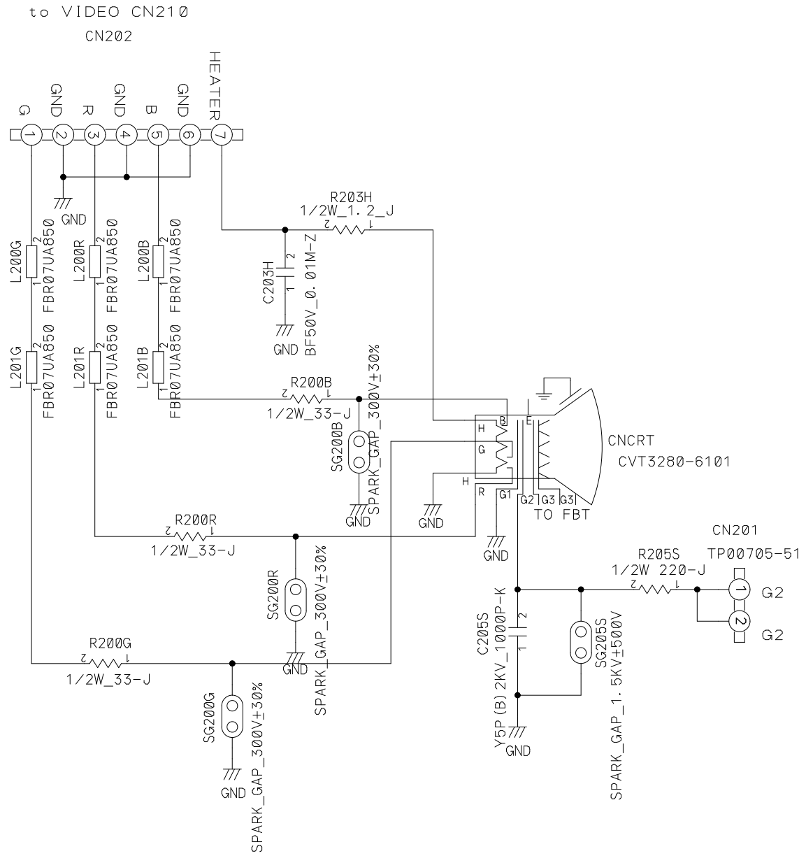
SCHMATIC DIAGRAM □ CRT □ DP2070SB(SH VERSION)
