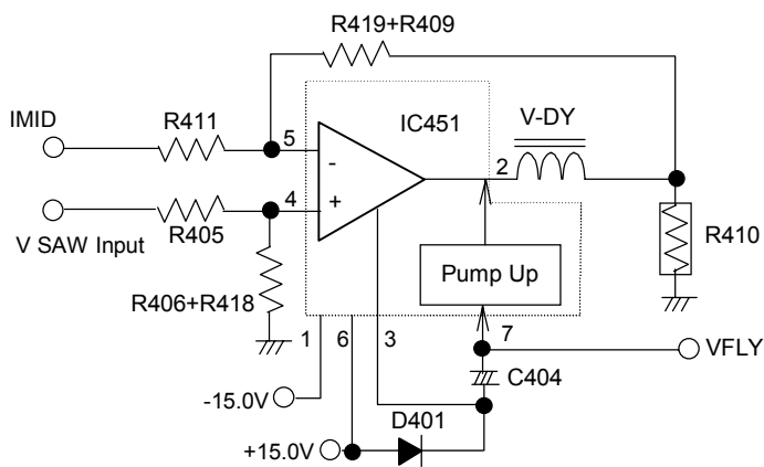
Fig. 3 Vertical output amplifier circuit
