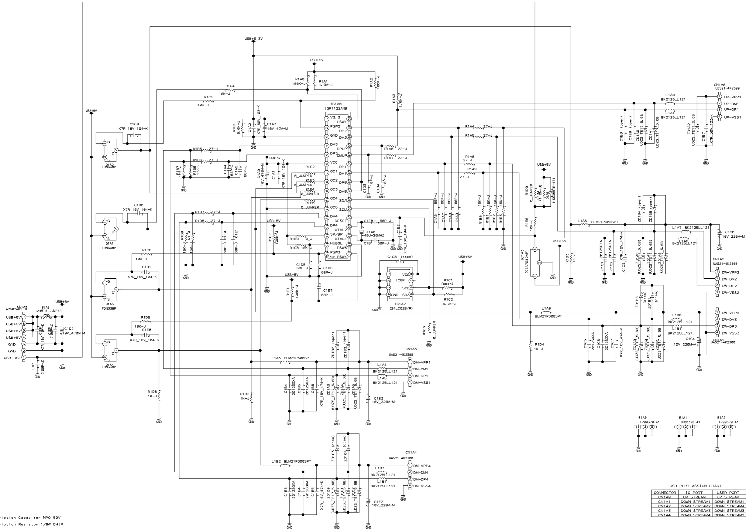
SCHEMATIC DIAGRAM □ USB-HUB □ DP2070SB(SH VERSION)
